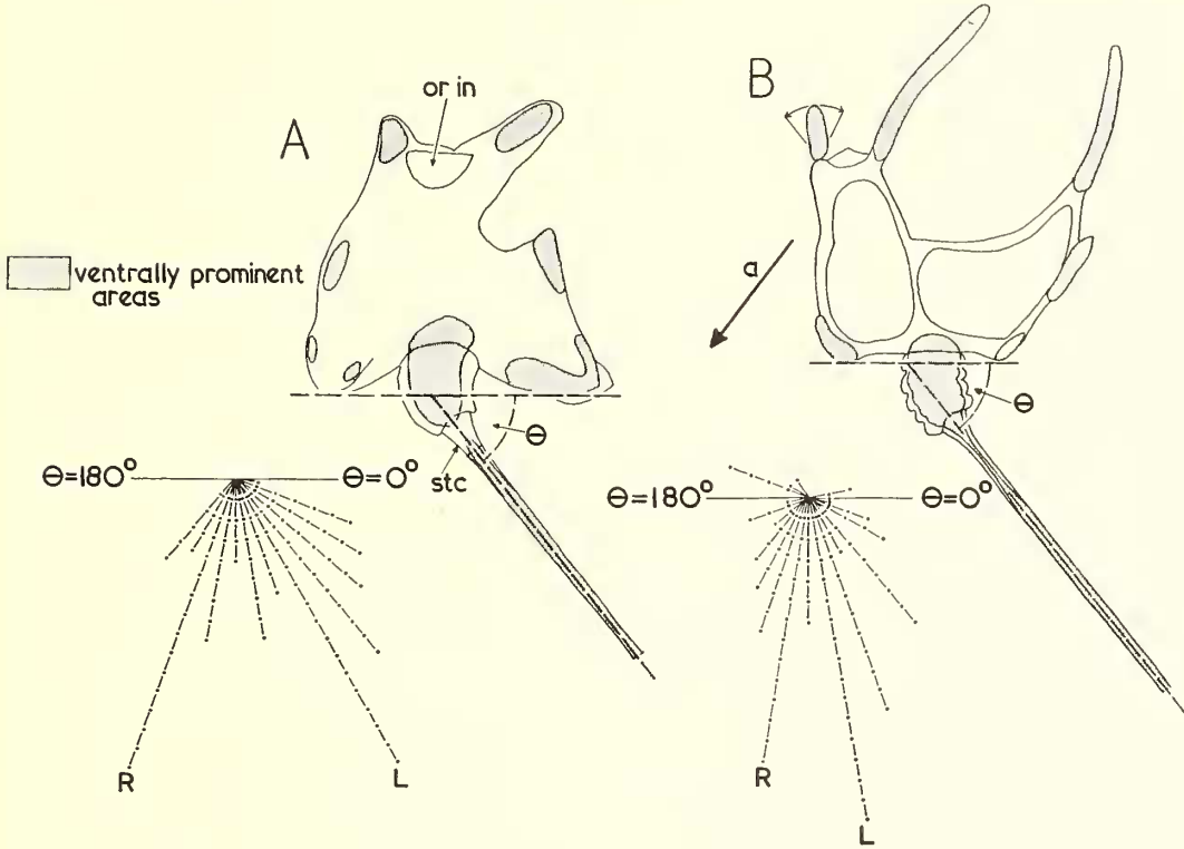
TEXT-FIG. 17. Ventrally prominent areas (stippled) and observed positions of stem in A, Ceratocystis perneri and B, Cothurnocystis elizae . or in = oral integument; stc = stylocone. R and L = especially frequent positions of stem to right and left. The arrow a indicates probable easiest direction of slip in Coth. elizae . In the histograms each dot indicates one specimen.
